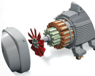
SR motor assembly utilizing standard IP55 housings. (L75SR shown)
