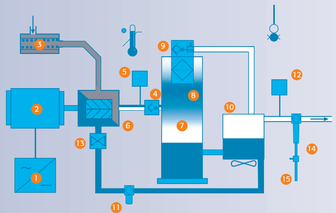
Typical Air/Oil Flow Diagram
